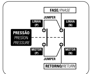
MONOFÁSICO INGLE-PHASE
